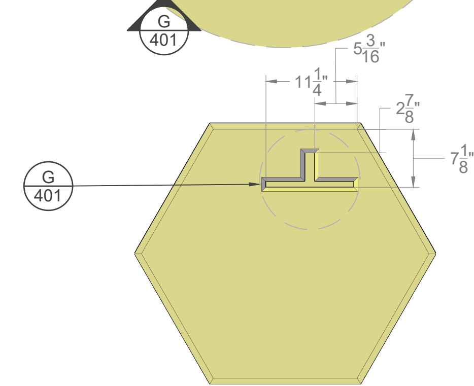
TOP: DECKING SLOT PLACEMENT
