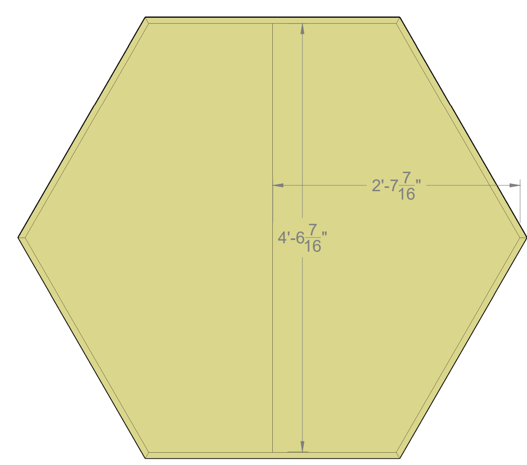
TOP: DECKING
