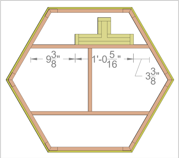
SLOT PLACEMENT
