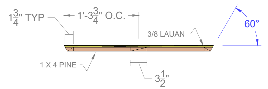
SEC. C
