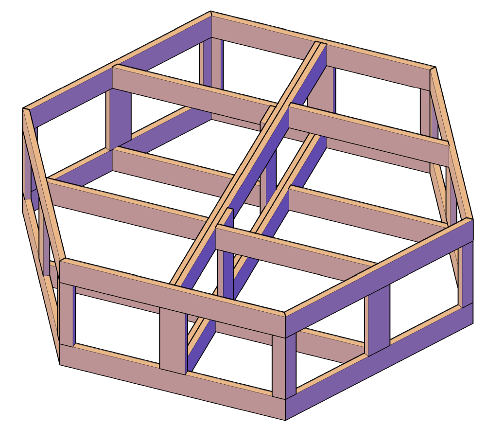
ISO: FRAMING
