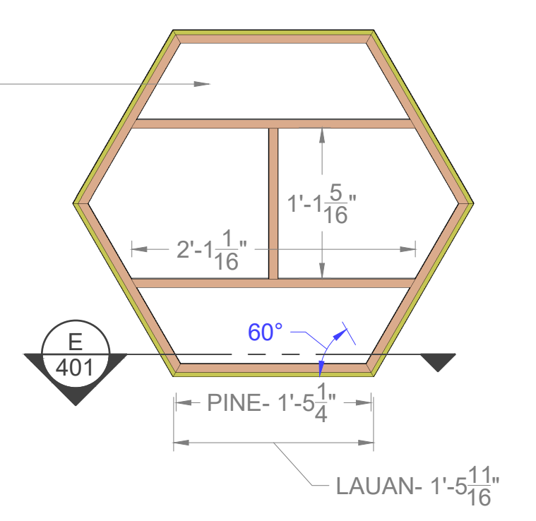
TOP: CUTTING
