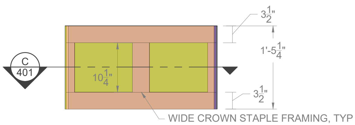
SEC. B
