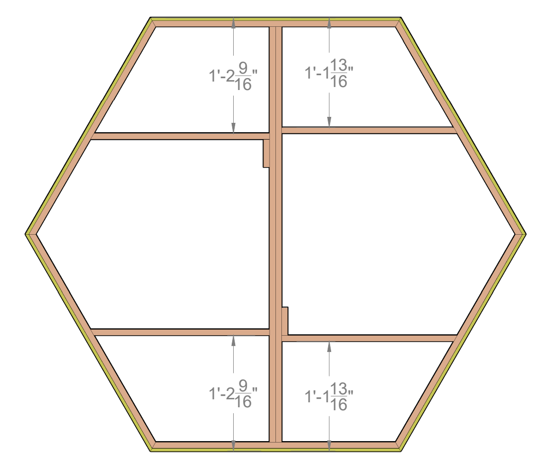
TOP: PLACEMENT
