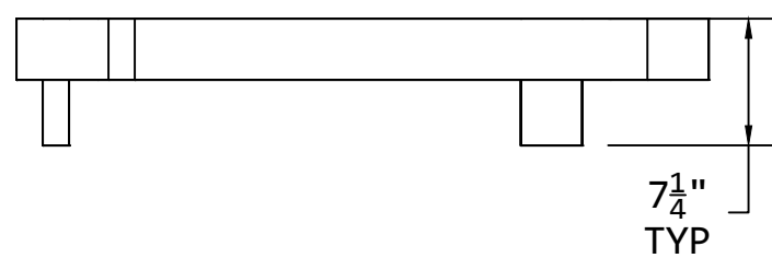
FRONT VIEW UPPER PLATFORM LEG LAYOUT
