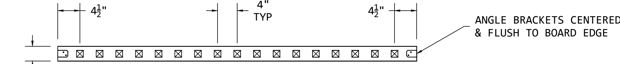
TOP SECTION VIEW
