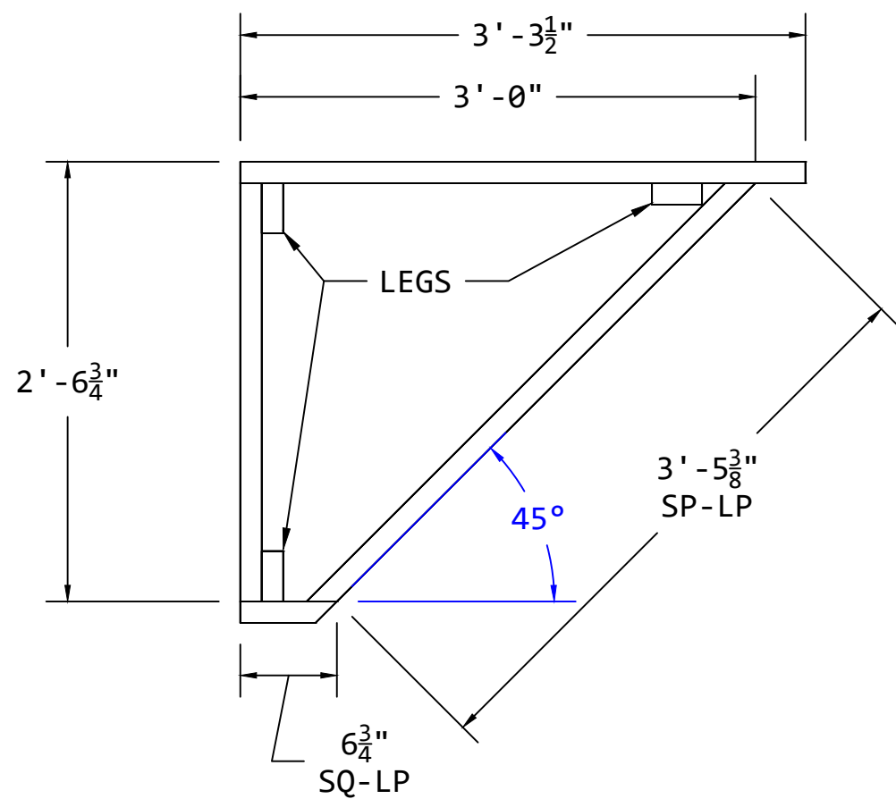
TOP VIEW FRAMING LAYOUT
