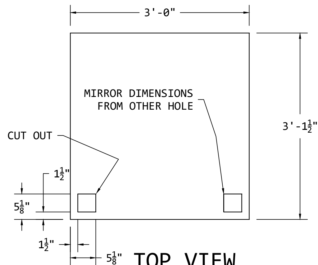
TOP VIEW LID LAYOUT
