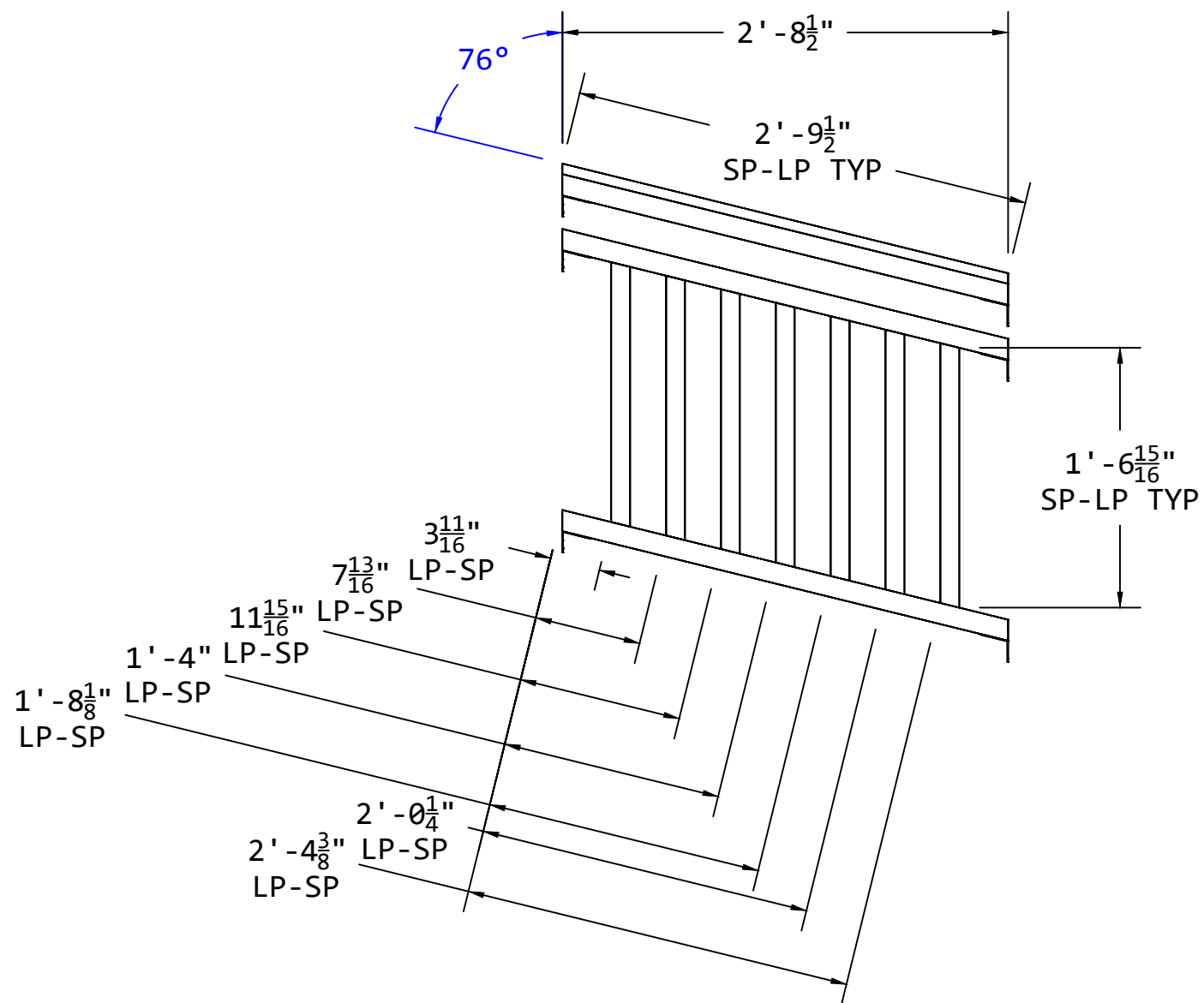
FRONT VIEW
