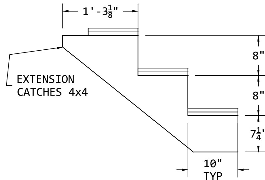
LEFT VIEW
