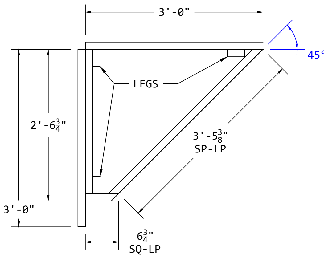
TOP VIEW FRAMING LAYOUT
