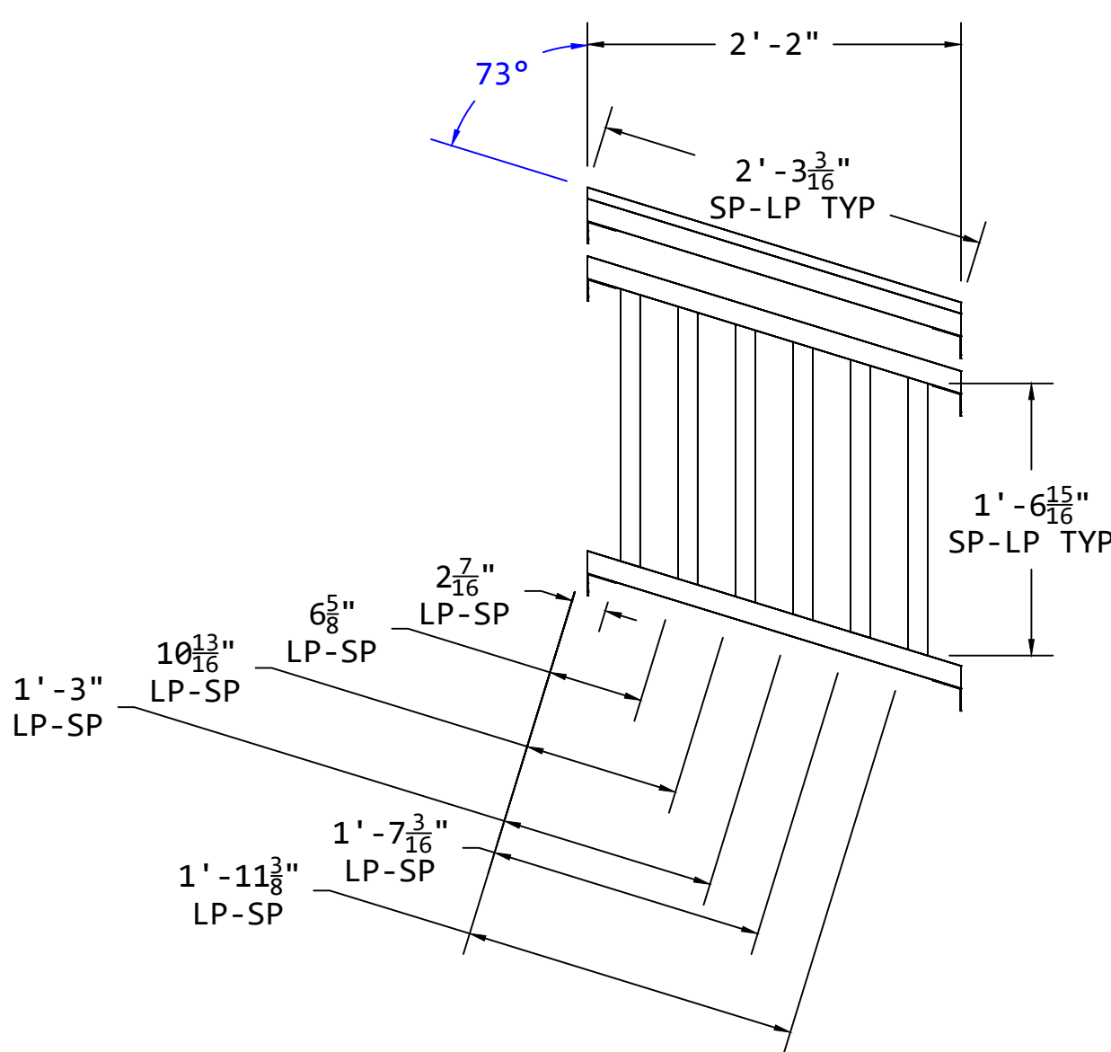
FRONT VIEW
