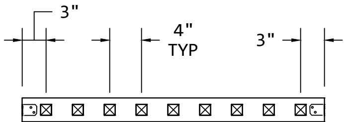
TOP SECTION VIEW
