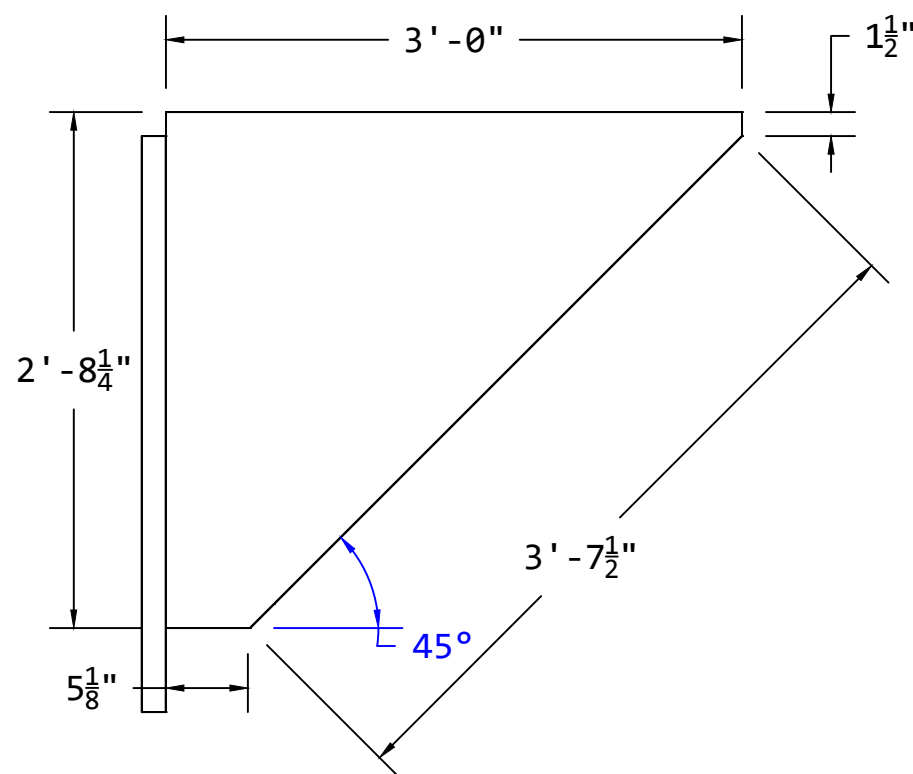
TOP VIEW LID LAYOUT
