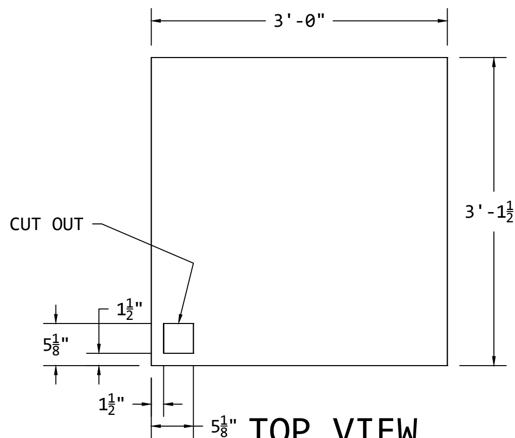
TOP VIEW LID LAYOUT
