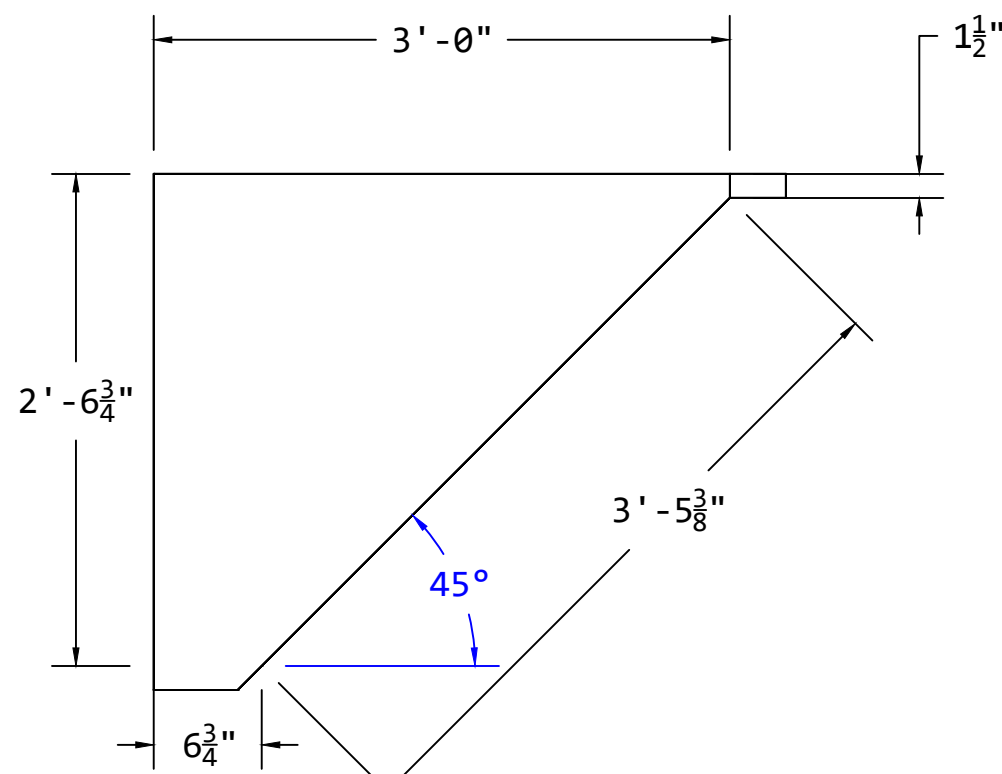
TOP VIEW LID LAYOUT
