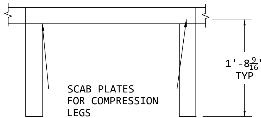
FRONT VIEW LOWER PLATFORM LEG LAYOUT
