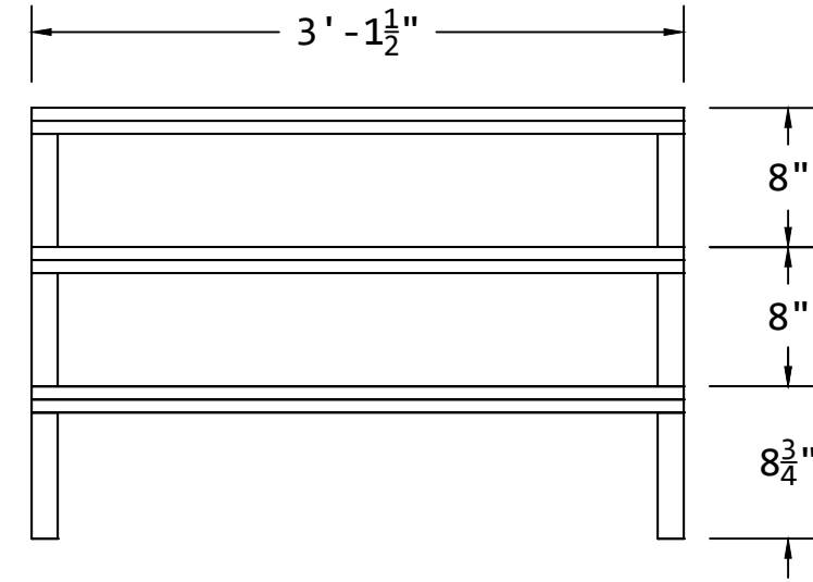
FRONT VIEW BUILD 1
