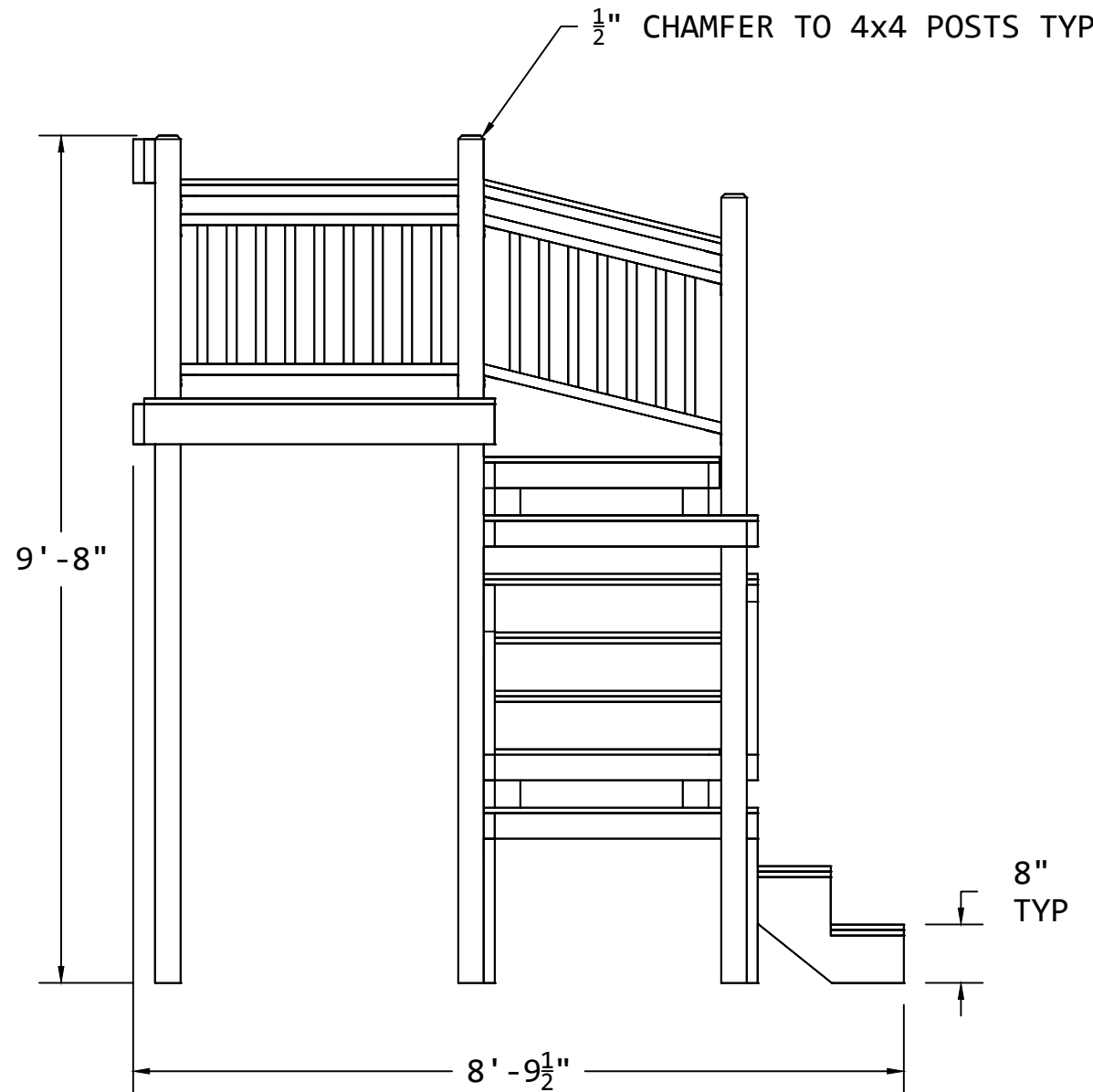
LEFT VIEW
