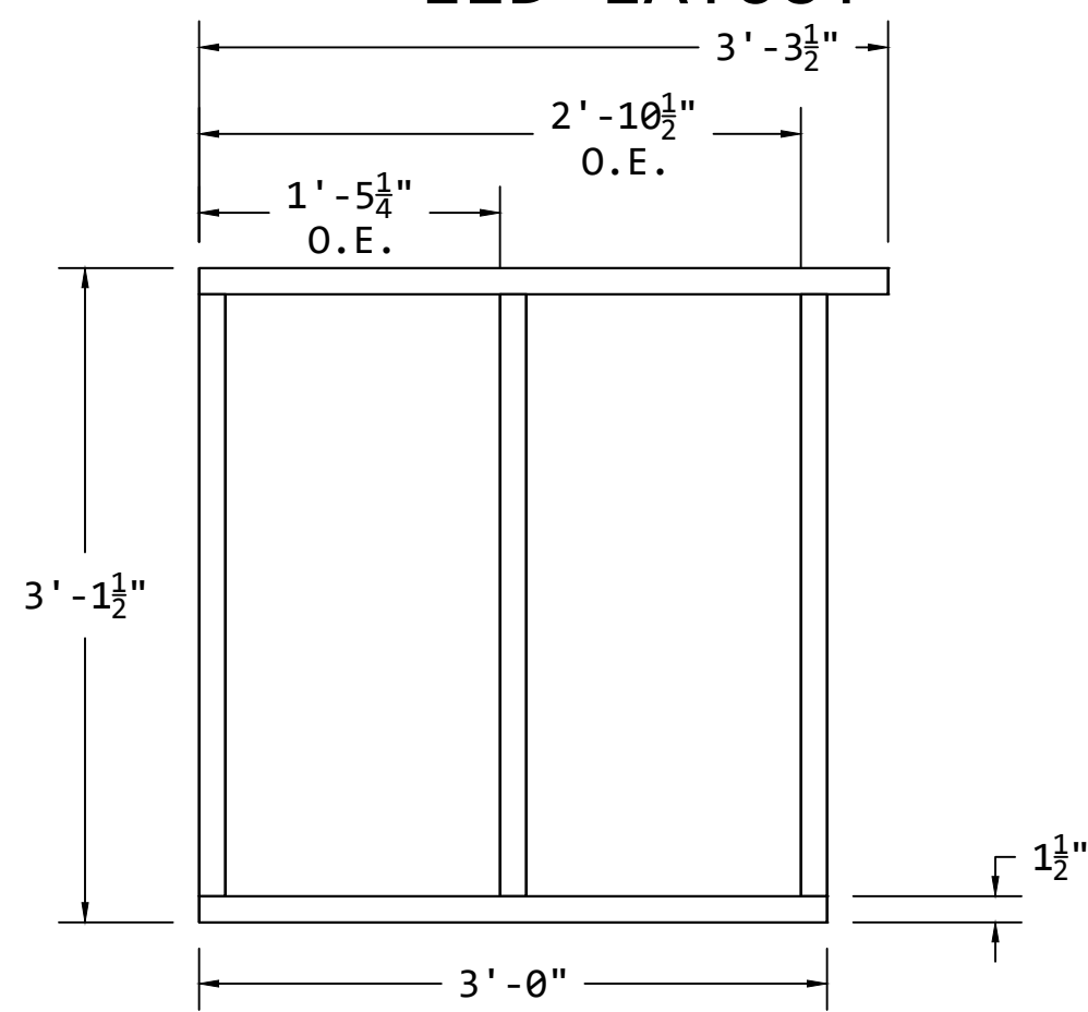
TOP VIEW LID LAYOUT
