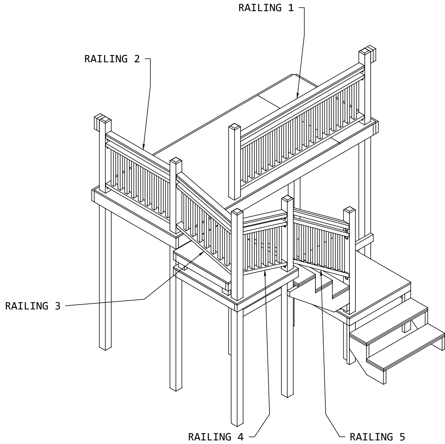
ISO VIEW ASSEMBLED LAYOUT SCALE: \frac{1}{2} "=1'-0"
