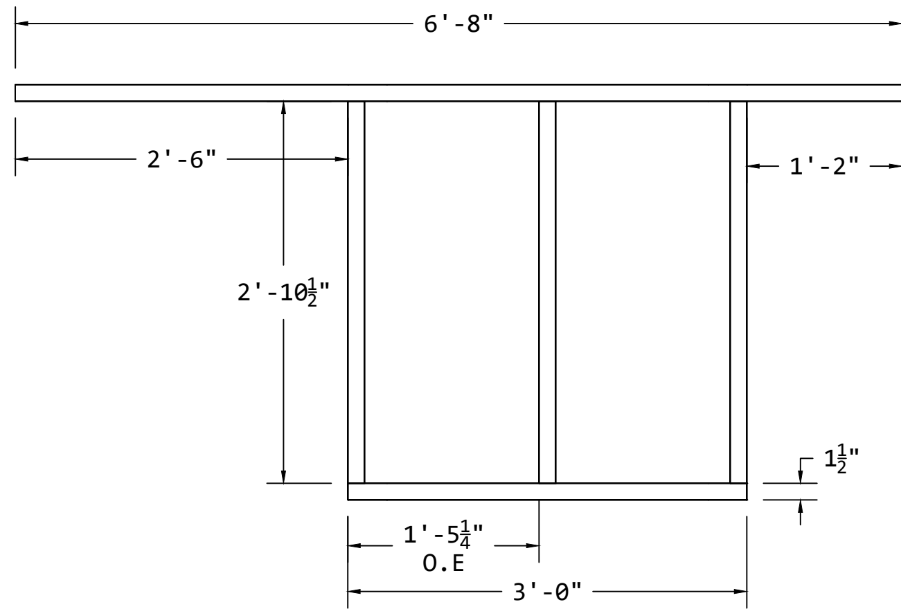
TOP VIEW FRAMING LAYOUT
