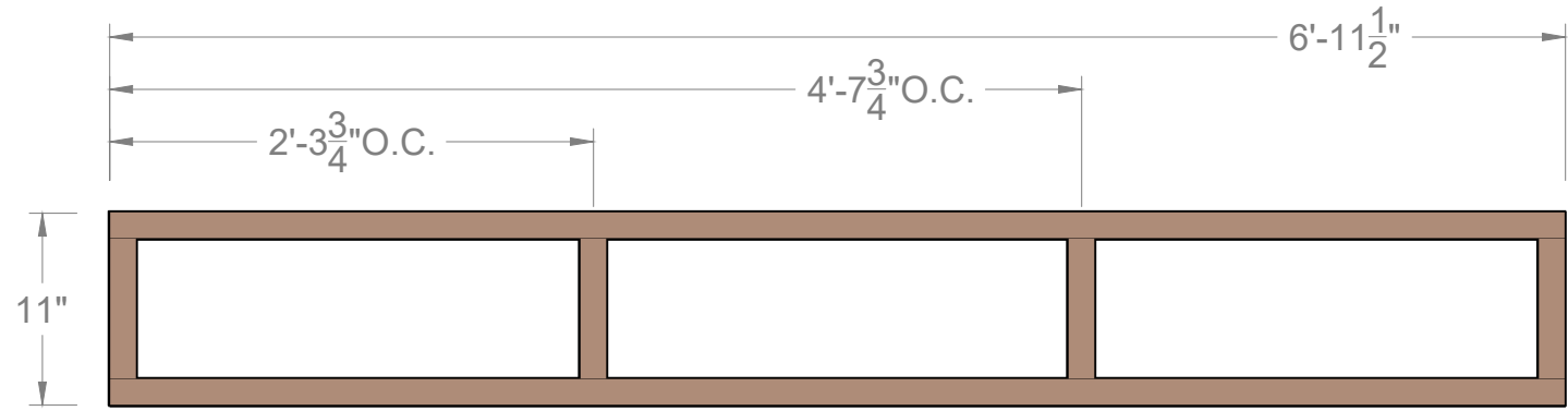
FRONT VIEW FRAMING LAYOUT
