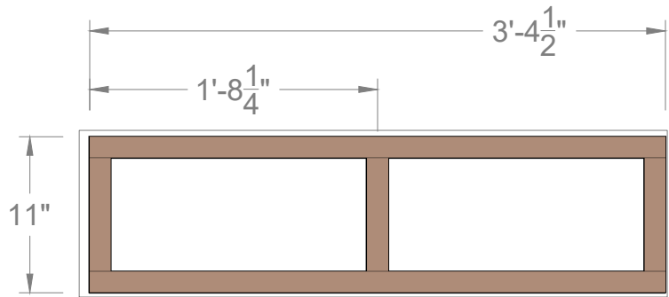
LEFT VIEW FRAMING LAYOUT
