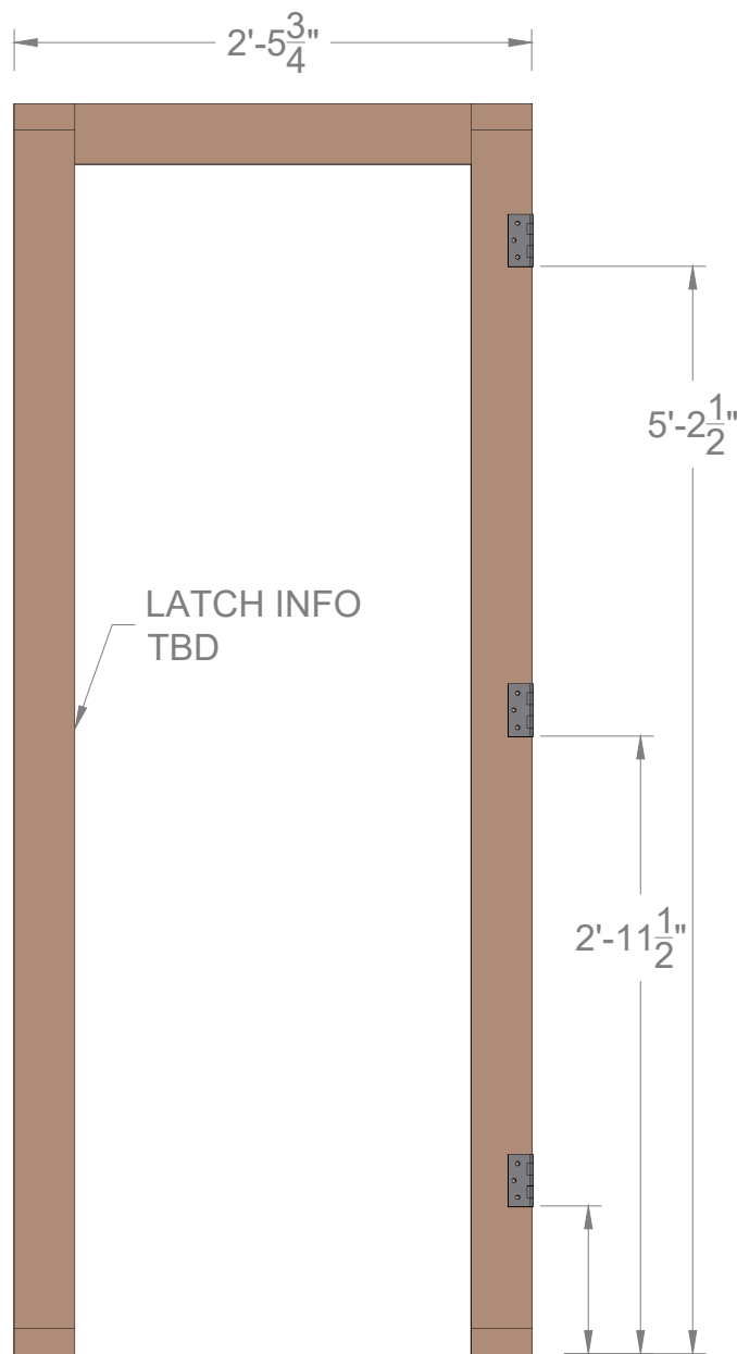
FRONT FRAMING LAYOUT
