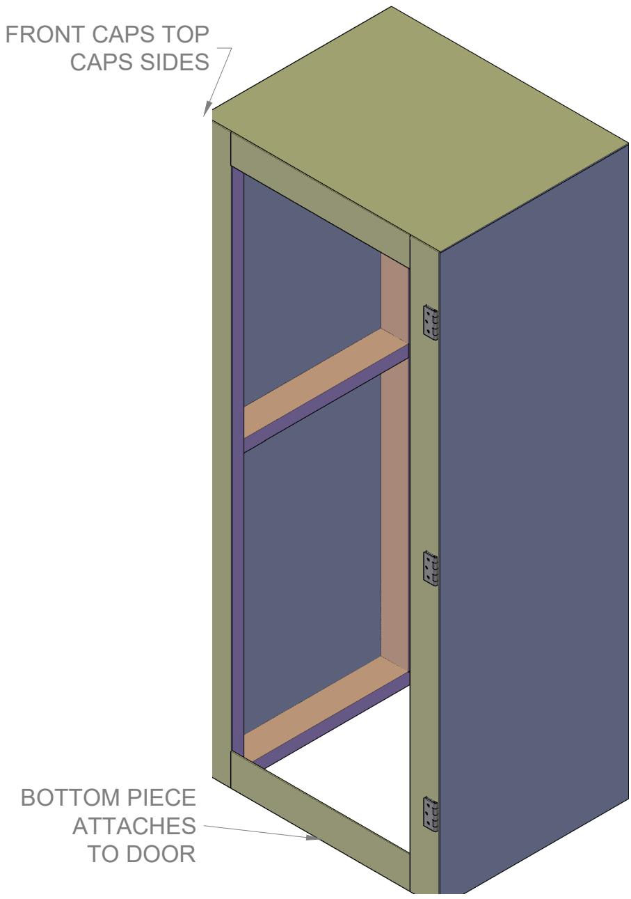
ISO FACING LAYOUT
