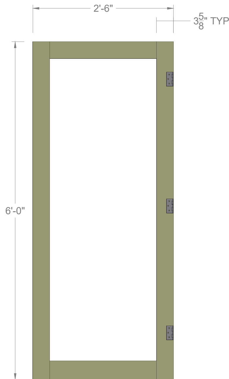
FRONT FACING LAYOUT
