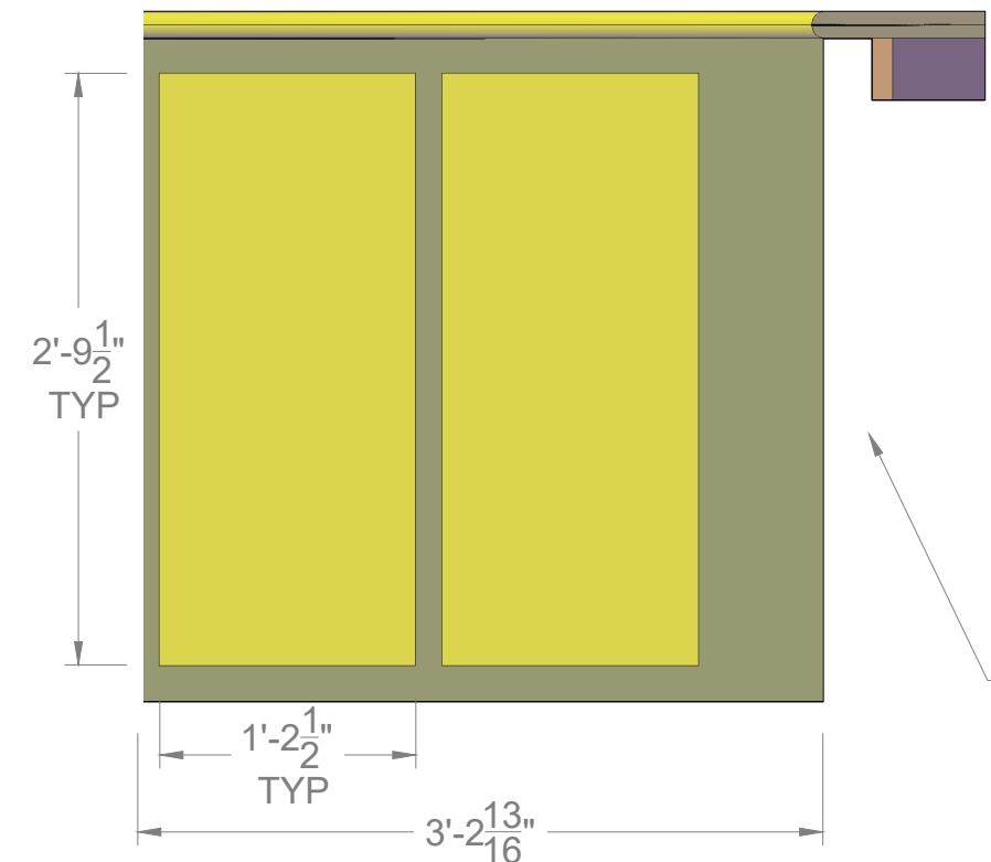
FRONT FACING LAYOUT
