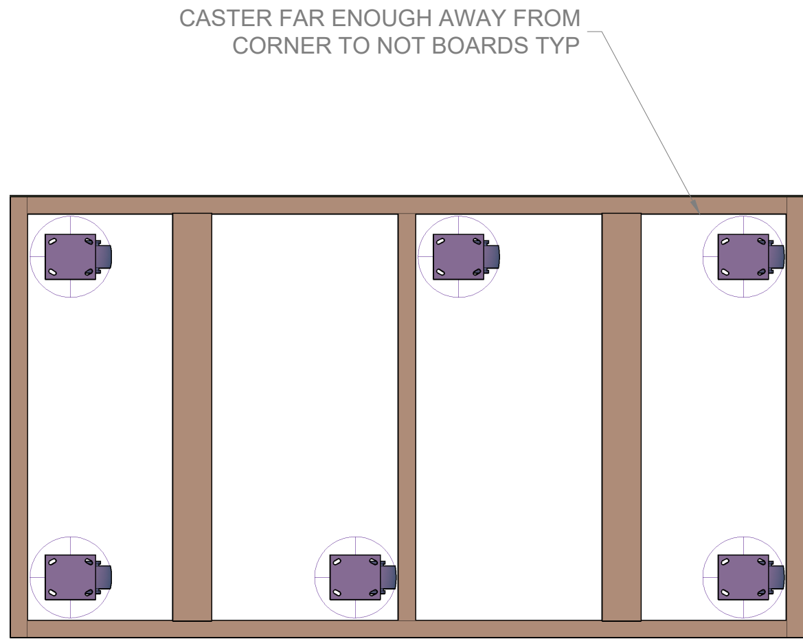
TOP VIEW CASTER LAYOUT DECK PREMADE
