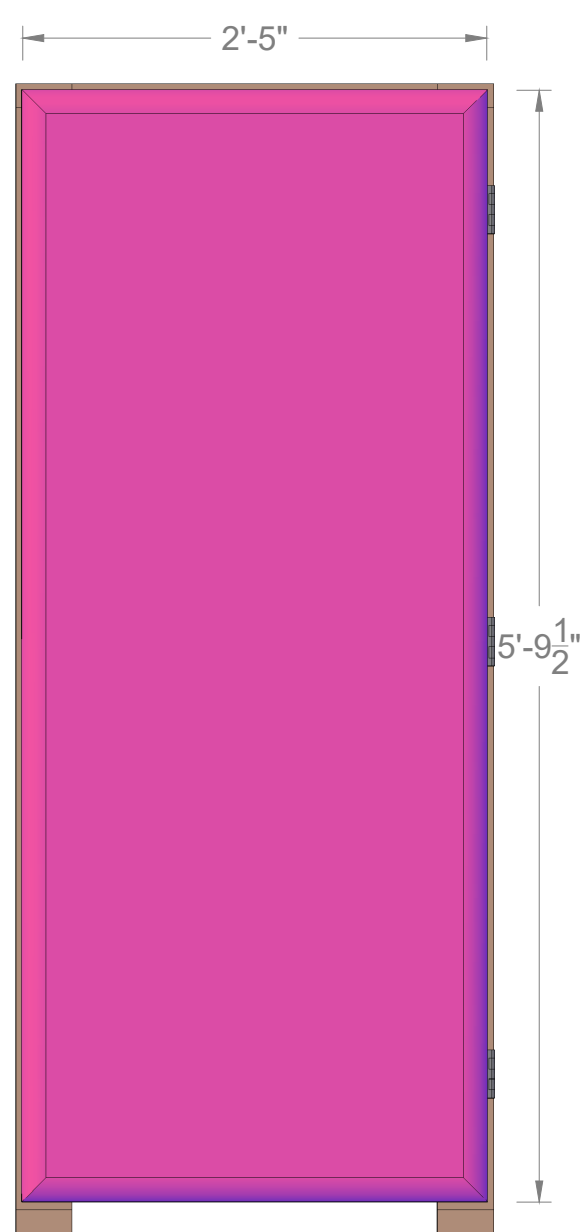
FRONT DOOR LAYOUT
