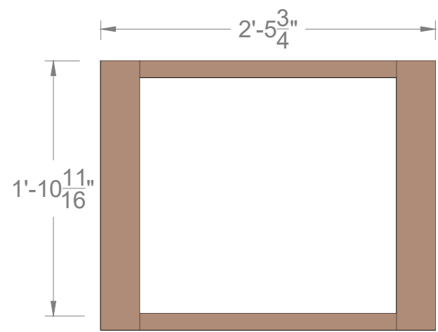
TOP FRAMING LAYOUT
