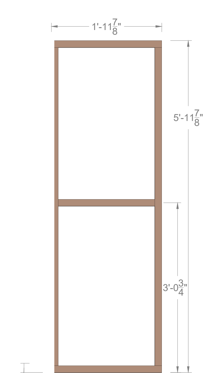
RIGHT FRAMING LAYOUT
