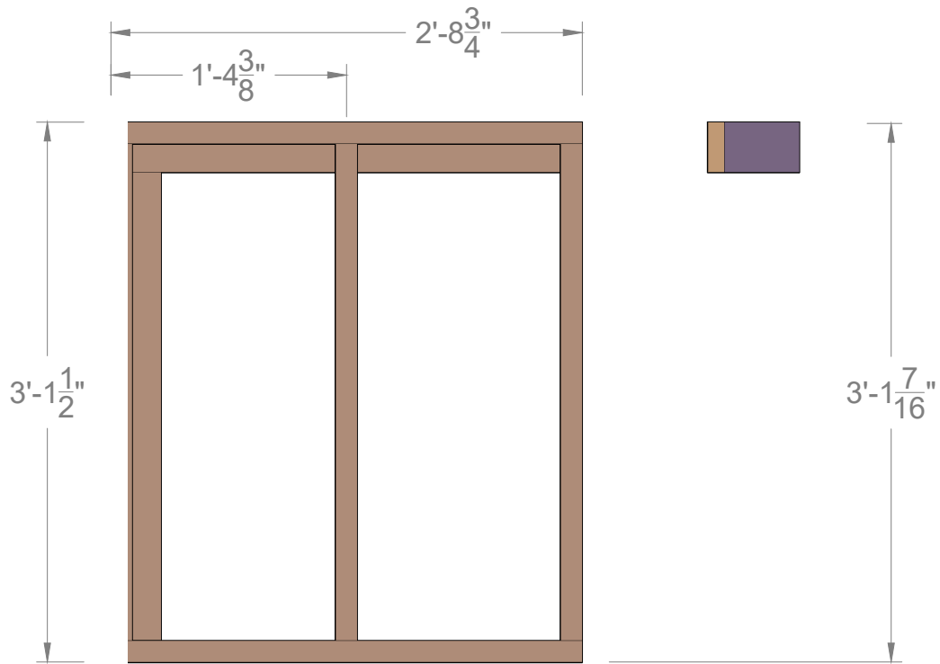
FRONT FRAMING LAYOUT
