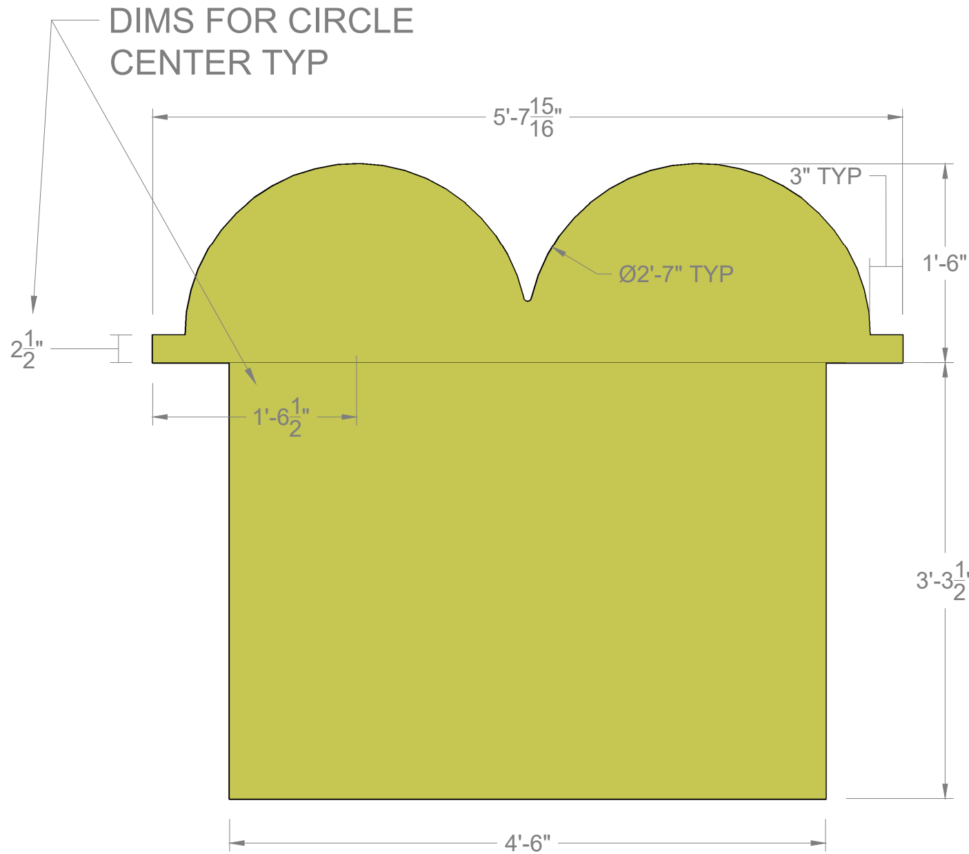
FRONT VIEW FACING LAYOUT
