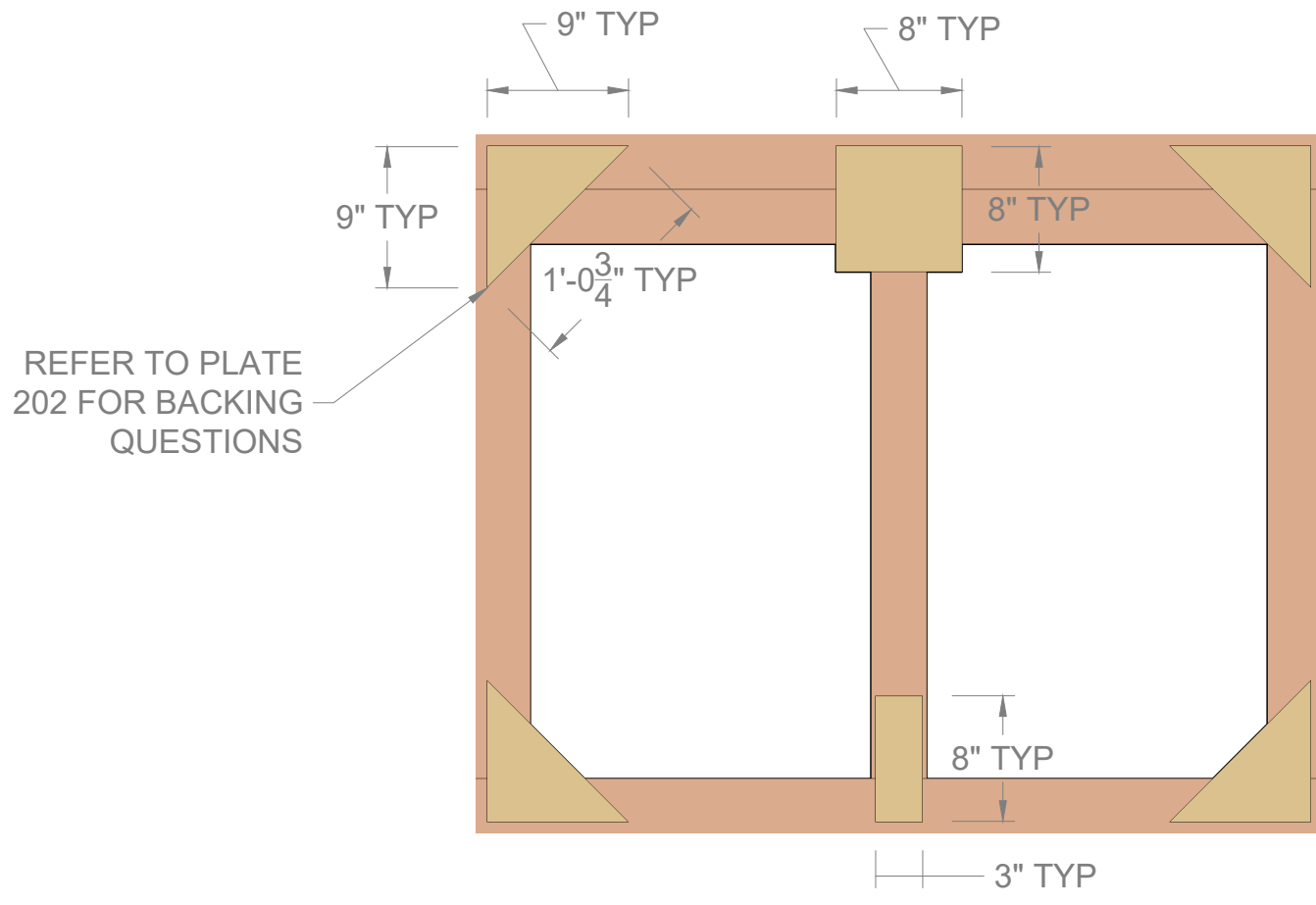
BACK VIEW BACKING LAYOUT
