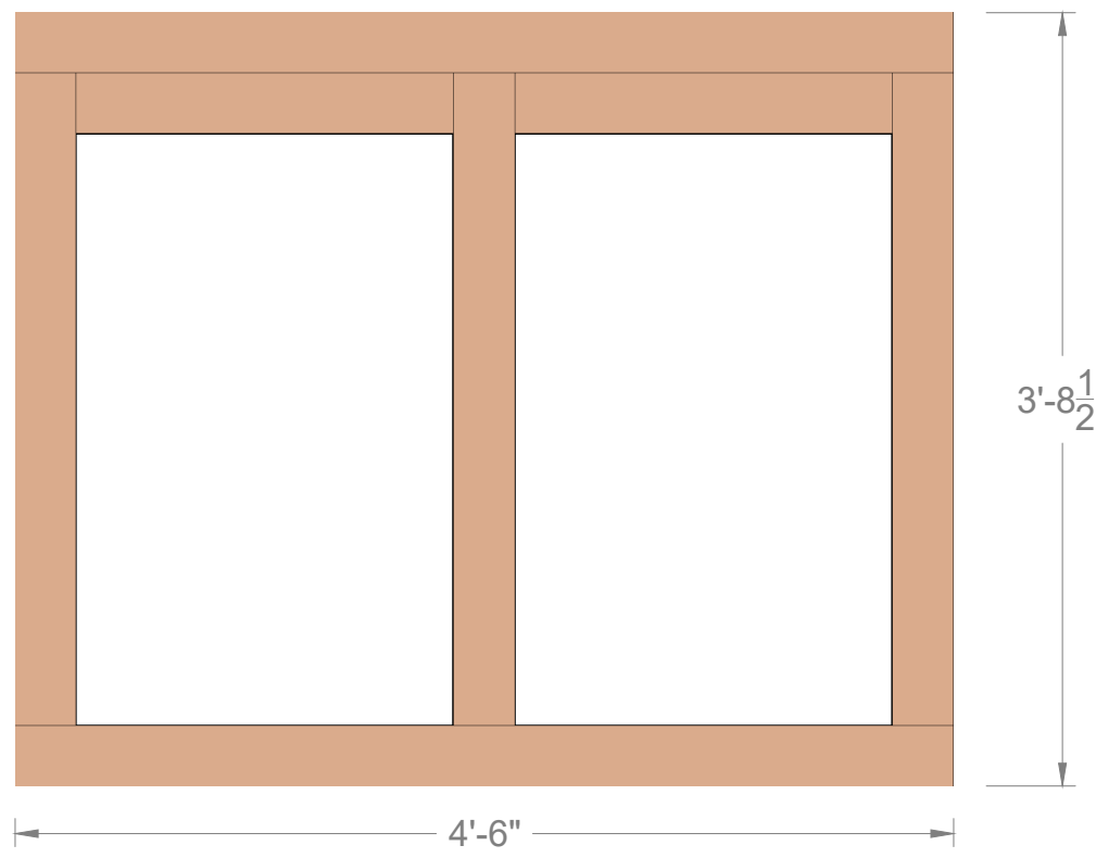
BACK VIEW FRAMING LAYOUT
