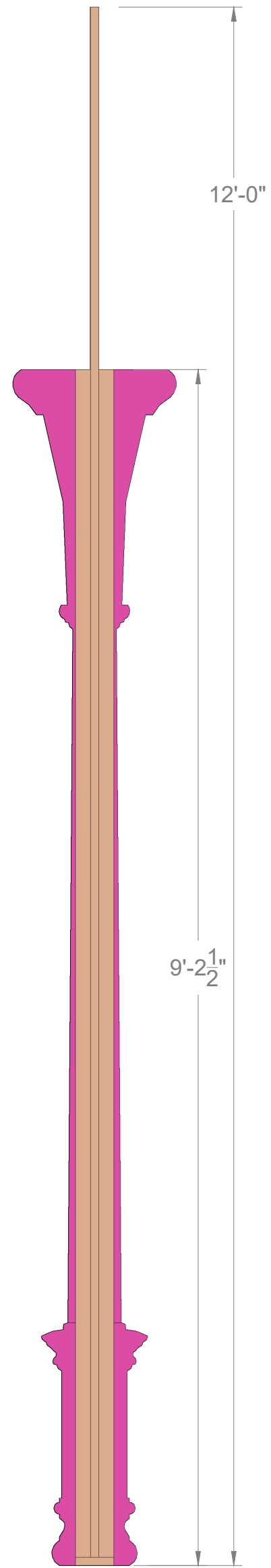
BACK VIEW FRAMING LAYOUT
