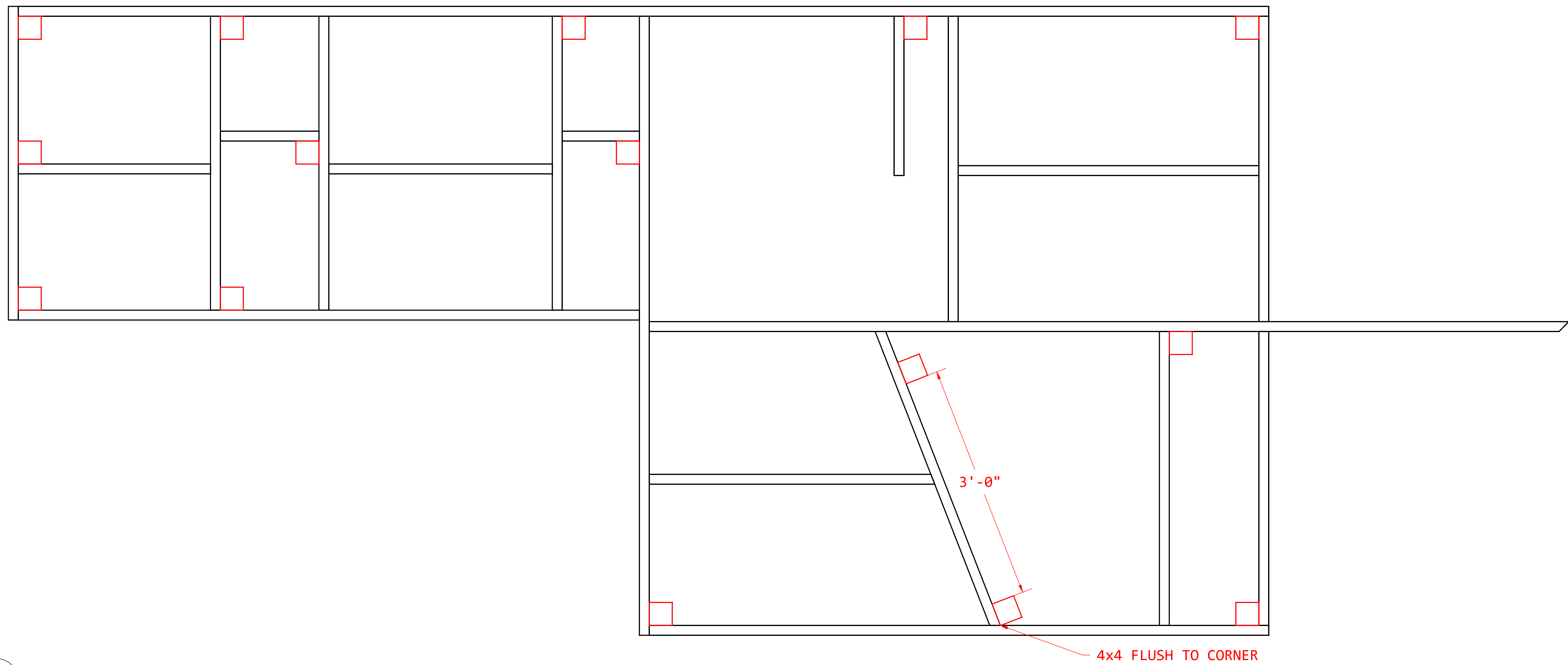
02 UPPER LEVEL PLATFORM – LEG 1 RIGHT 02 – 4x4 PLACEMENT STAGE 1 – 4x4 CUT TO LENGTH THEN ATTACHED FLUSH TO FRAMING EDGE & STICKING DOWN – GLUE & SCREW 1"=1'-0"
