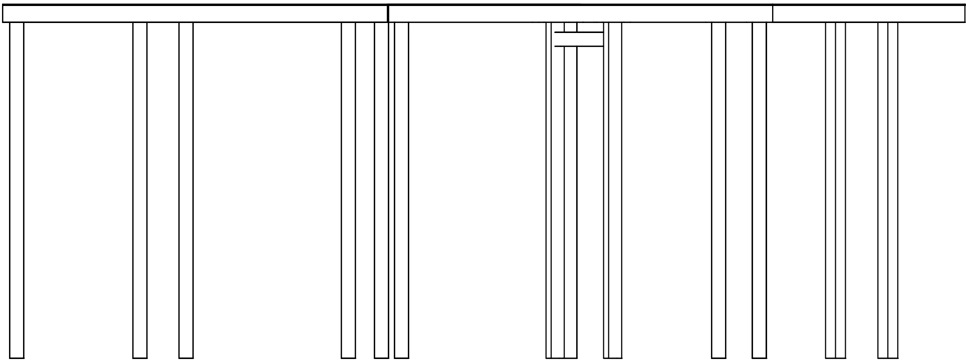
04 UPPER LEVEL PLATFORM OVERVIEW FRONT 01 - 2x4 FRAMING, 3/4" CDX PLY LID, 1/4" MASO FACING 1/2"=1'-0" - WEIGHT: 996# - DO NOT BUILD FROM THIS PLATE
