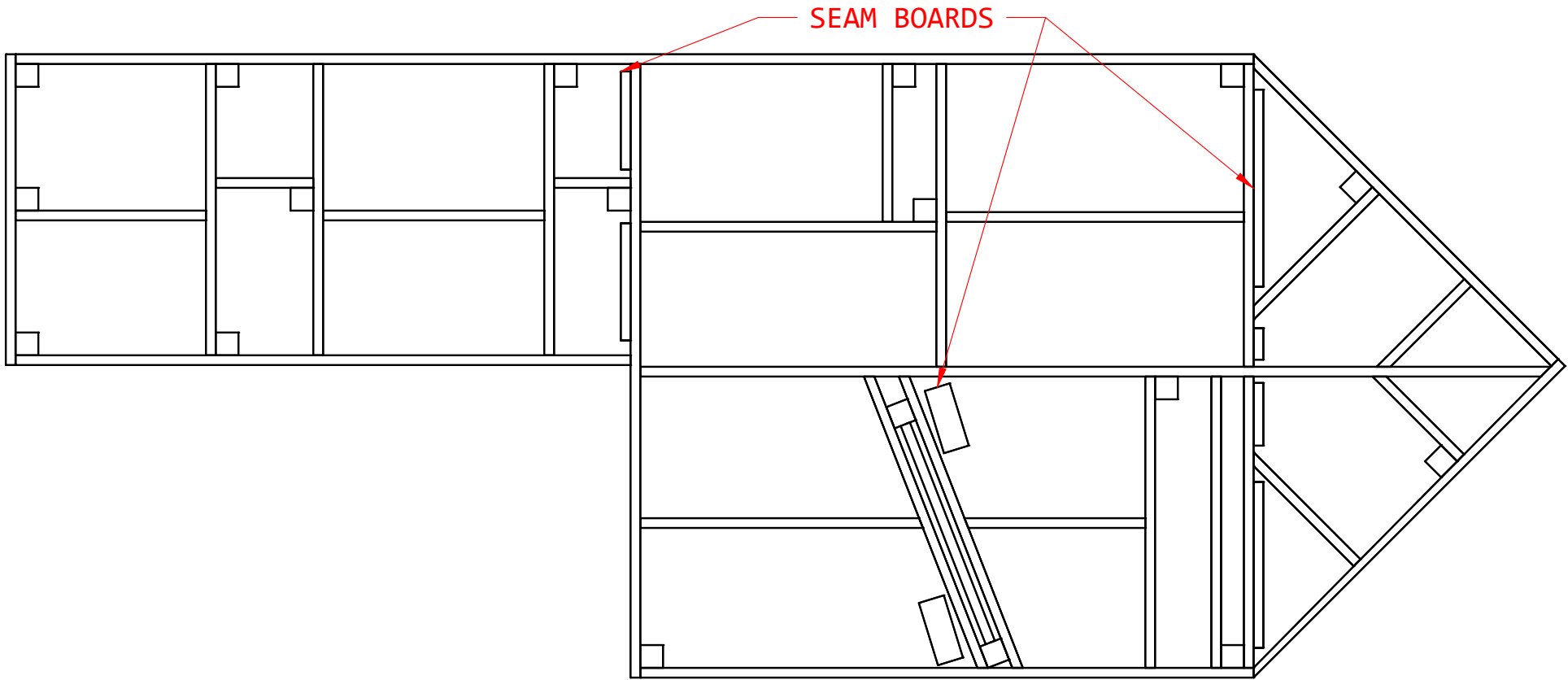
03 UPPER LEVEL PLATFORM FRAMING TOP 01 - 2x4 FRAMING, 3/4" CDX PLY LID, 1/4" MASO FACING 1/2"=1'-0" - WEIGHT: 996# - DO NOT BUILD FROM THIS PLATE
