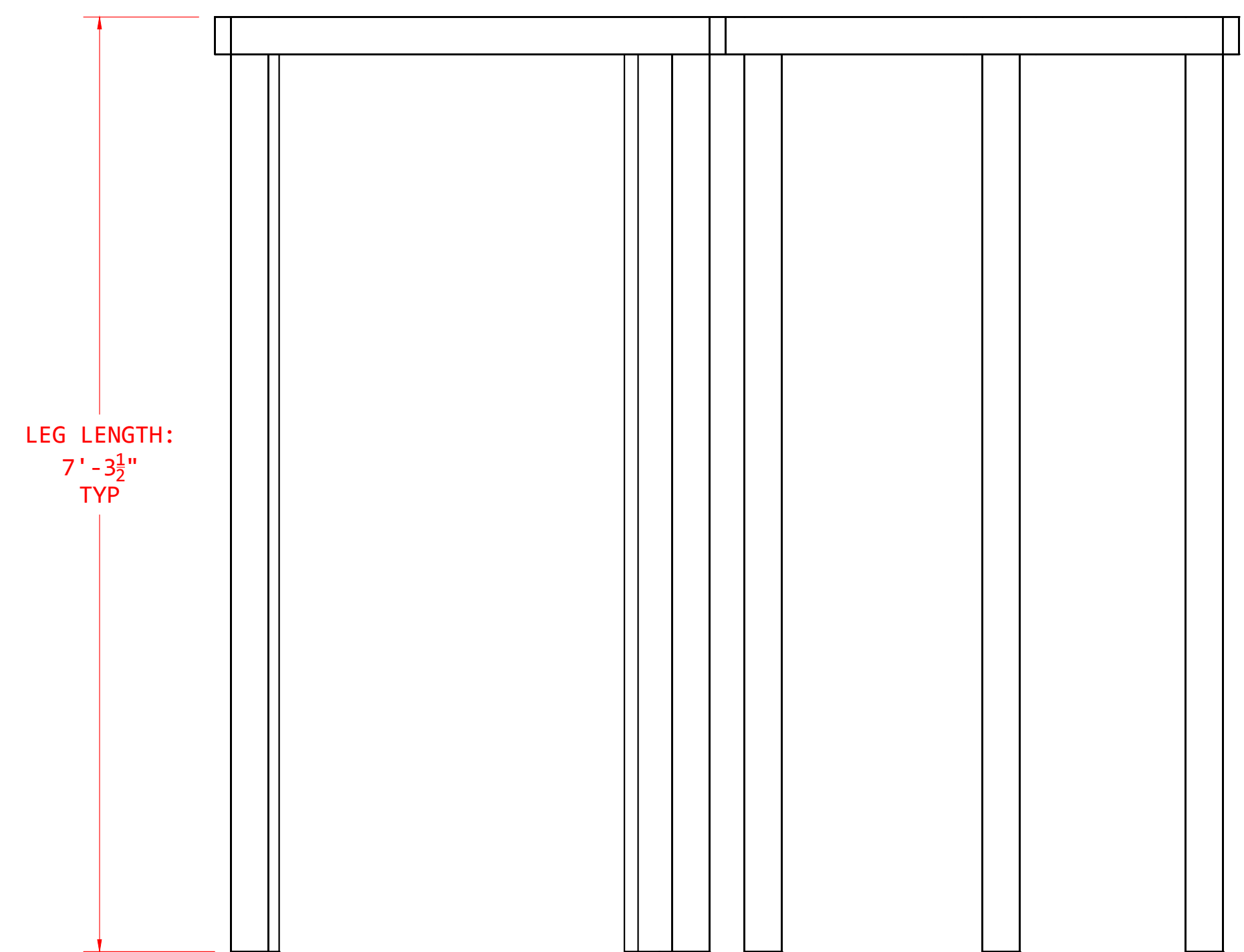
03 UPPER LEVEL PLATFORM – LEG 1 RIGHT 02 – 4x4 PLACEMENT STAGE 1 – 4x4 CUT TO LENGTH THEN ATTACHED FLUSH TO FRAMING EDGE & STICKING DOWN – GLUE & SCREW 1"=1'-0"
