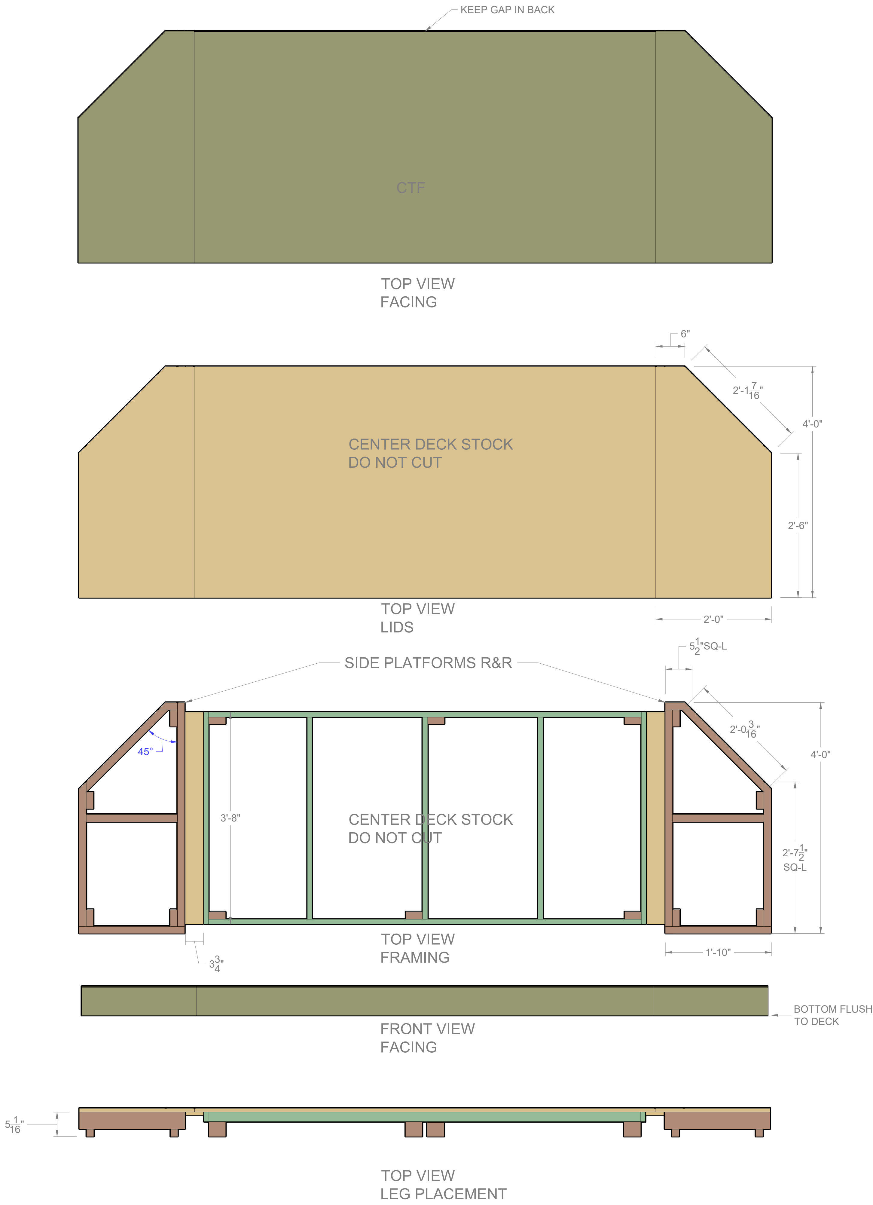
A 201 ENTRANCE PLATFORM NOTES: 2x4 FRAMING & LEGS, 3/4" CDX PLY LID, 3/16" MASO TOP FACING, 1/8" SIDE FACING SCREW LIP & SHELF PLATFORM CONNECTION - 3/4" CDX PLY SCREW FRAMING & LEGS 1/4" NARROW CROWN STAPLE FACING CTF FACING, TOP LIDDING SIDES MIDDLE DECK IS STOCK SCALE: 1"=1'-0"
