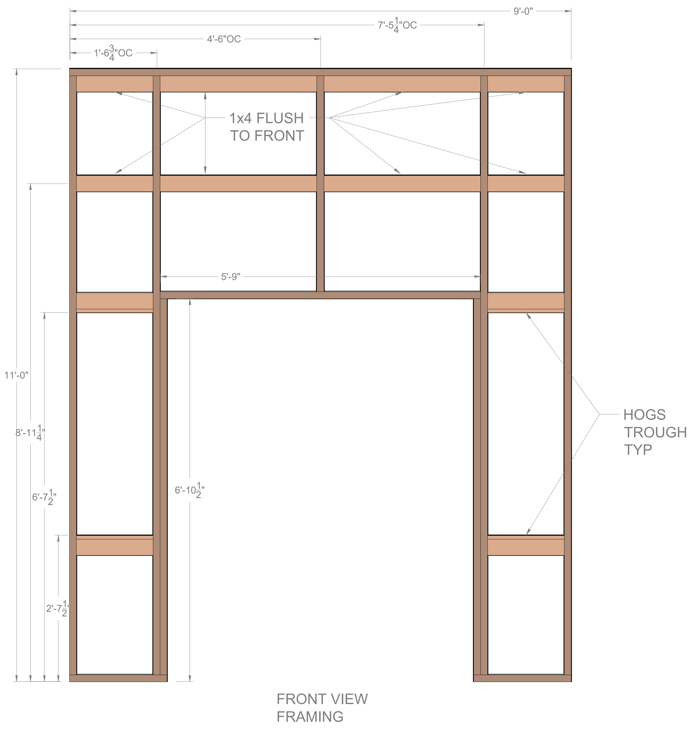
B 201 ENTRANCE CENTER WALL NOTES: 2x4 FRAMING, STOCK HOGS TROUGH FACING, 1/4" LAUAN FACING SCREW FRAMING, GLUE & 1/4" NARROW CROWN STAPLE FACING REFER TO A202 FOR FACING SCALE: 1"=1'-0"
