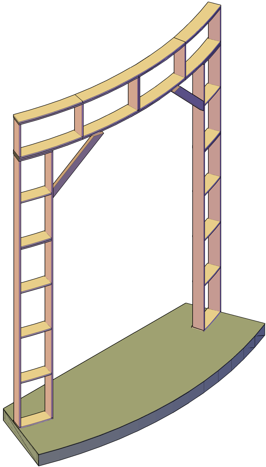
ISO FRAMING OVERVIEW SCALE: \frac{1}{2} " = 1'-0"
