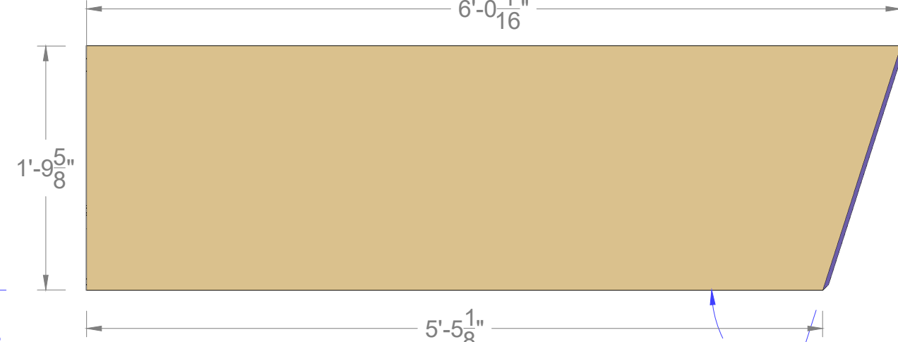
FRONT VIEW: PLY LAYOUT
