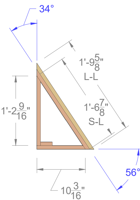
LEFT VIEW: FRAMING LAYOUT
