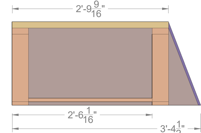
BACK VIEW: FRAMING LAYOUT
