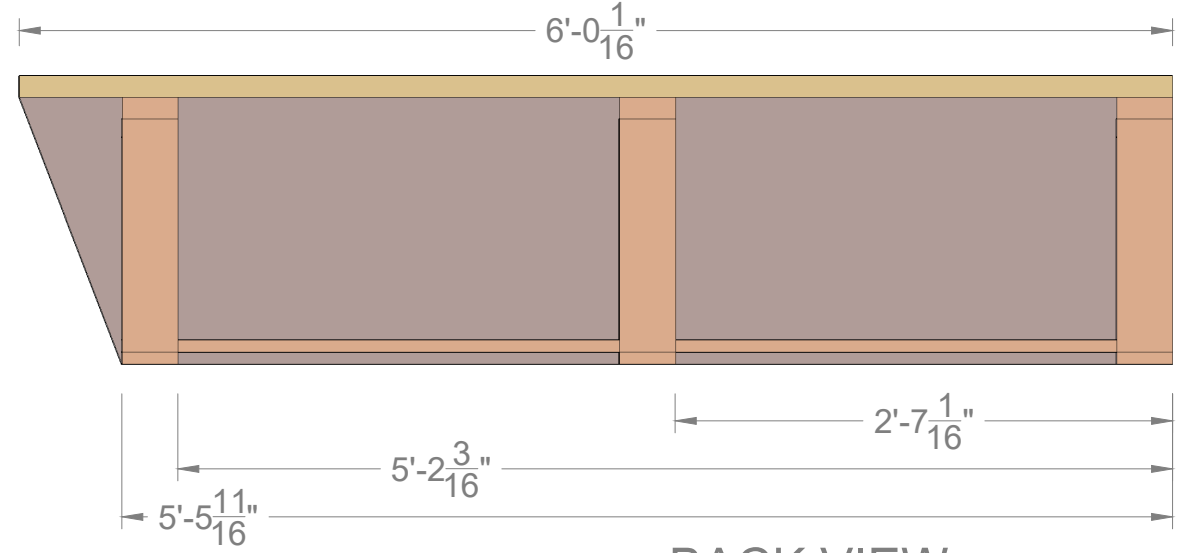
BACK VIEW: FRAMING LAYOUT
