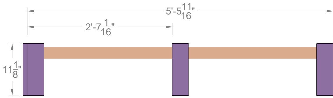
TOP VIEW: FRAMING LAYOUT
