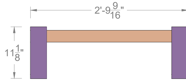
TOP VIEW: FRAMING LAYOUT
