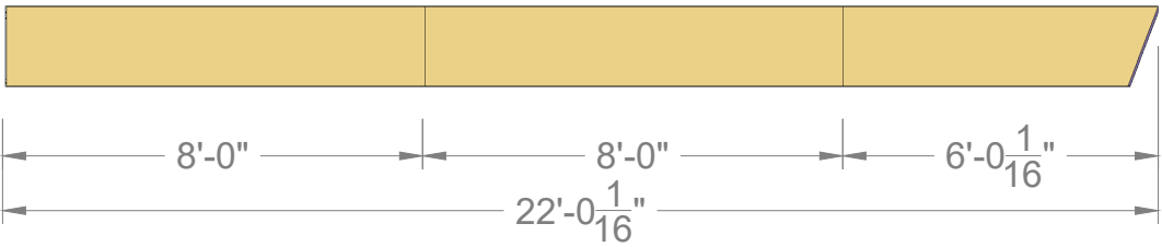
FRONT VIEW
