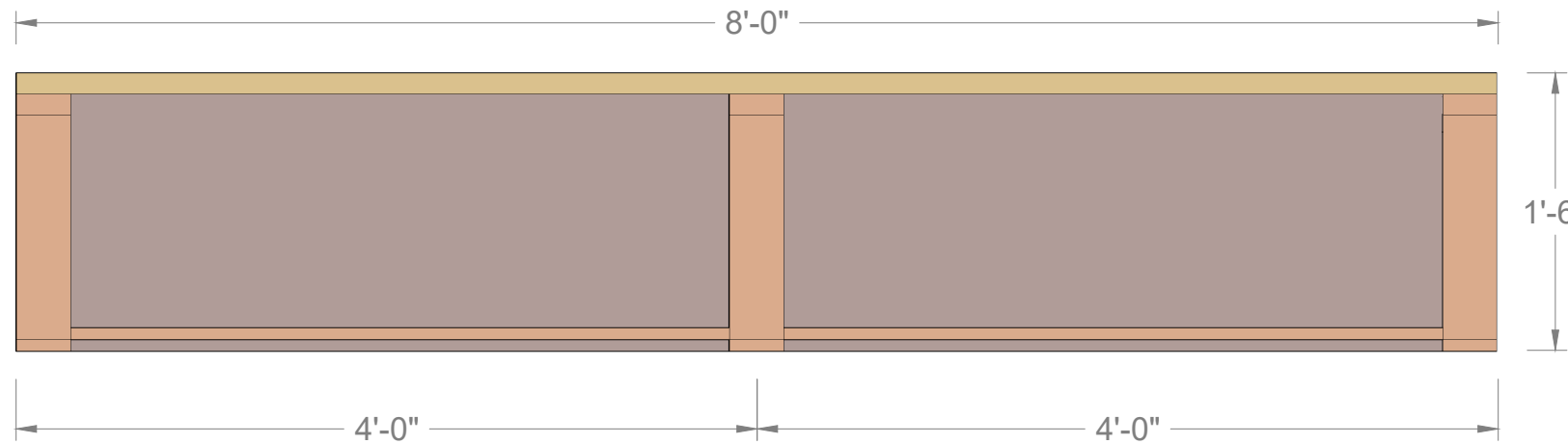
BACK VIEW: FRAMING LAYOUT
