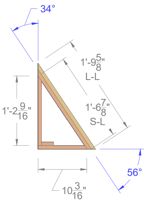
LEFT VIEW: FRAMING LAYOUT
