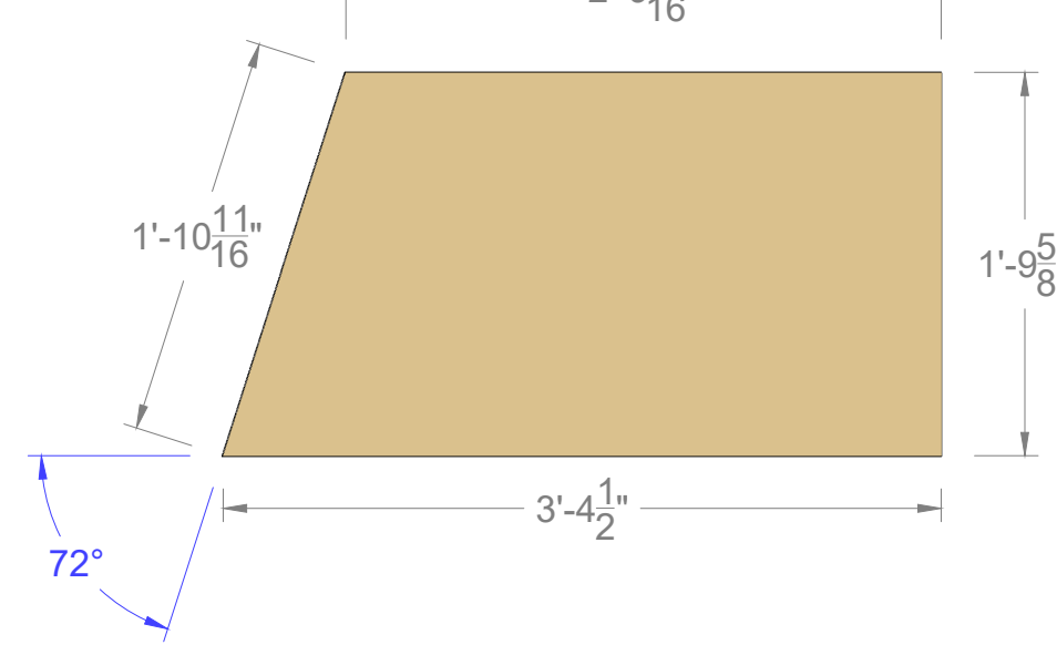
FRONT VIEW: PLY LAYOUT
