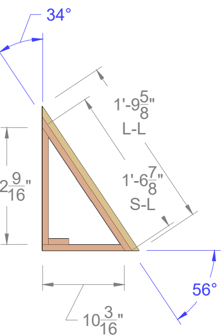
LEFT VIEW: FRAMING LAYOUT
